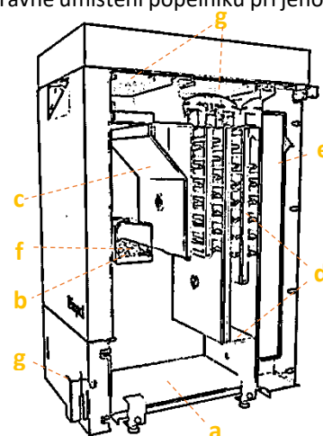
Biopel 10-40kW
